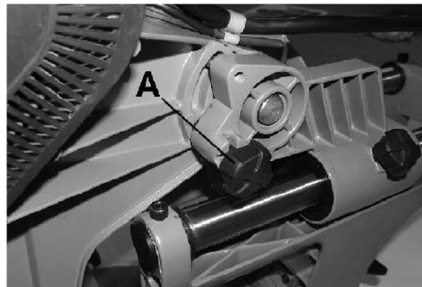
Obr. 5: Aretace hlavy pily
